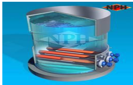
Pipe Insert Heaters
