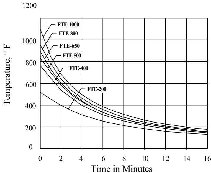
Surface Temperature Cool-Down Time: Single Emitter in 70 °F (21 °C) Ambient
